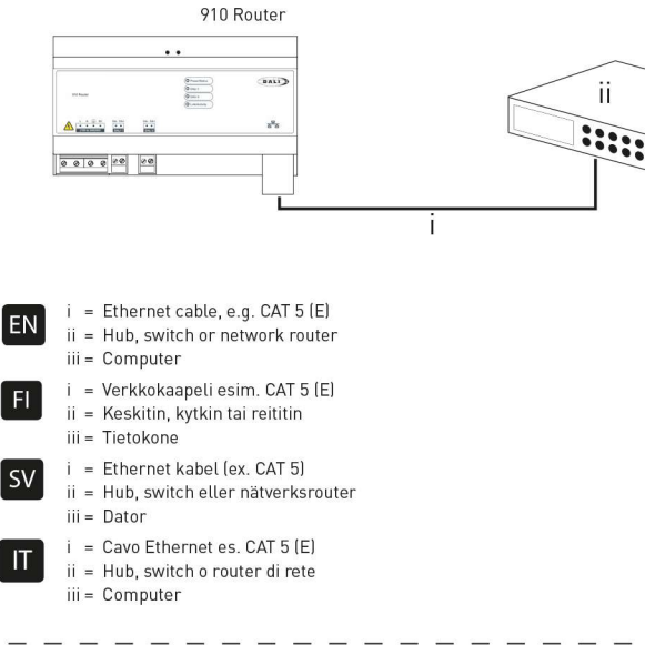
3b: ETHERNET CONNECTION
