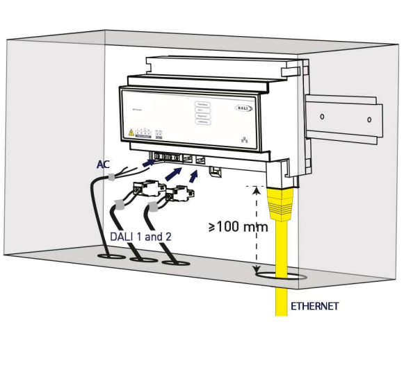
3b: ETHERNET CONNECTION
